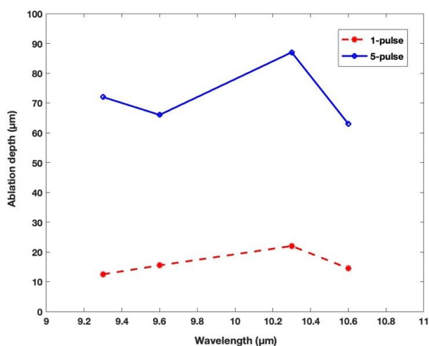
Figure 9. Depth of ablation at different wavelengths of \text{CO}_2 laser for one pulse and five pulses on dentin with water spray cooling
