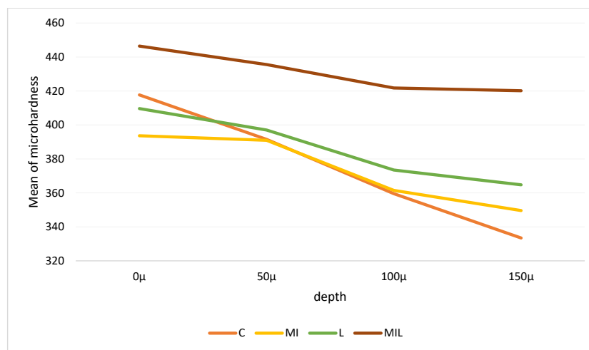
Figure 2. The Comparison of the Microhardness of Different Groups at Different Depths.
