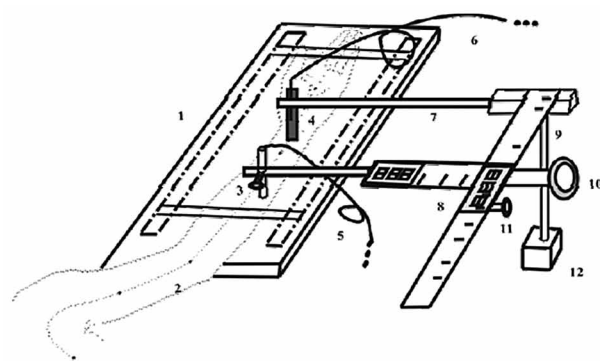
Figure 3. Diagram of the precise device for locating measurement points.
