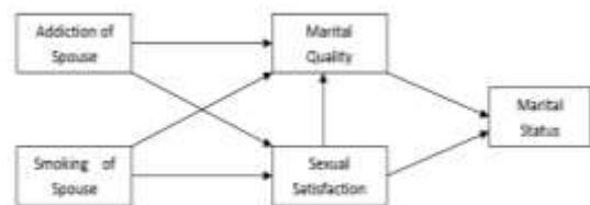
Figure2. The Theoretical Path Model for Variables Predicting Marital Status.
