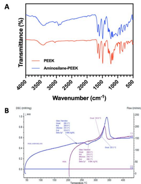
Figure 1- (a) FTIR spectra and (b) DSC graphs of PEEK and APTES grafted PEEK particles
