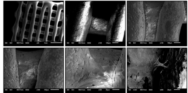
Figure 4- SEM micrographs of the cells attached on the 3D printed composite scaffolds at different magnifications
