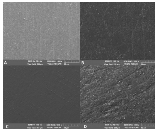
Figure 2- SEM micrograph of Gradia Direct surface polished with different finishing and polishing systems (x1000 magnification). (A) Control (Mylar); (B) Polished with Sof-Lex; (C) Polished with Super Snap; (D) Polished with Jiffy
