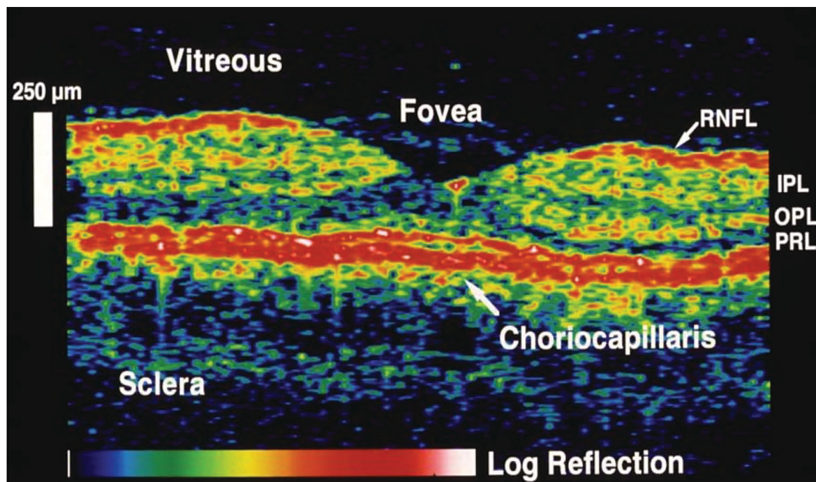
Figure 2: The initial in vivo OCT image of a healthy human retina demonstrates an approximate axial resolution of 15 \mu\text{m} (in tissue) at a wavelength of approximately 840 nm (adopted from Swanson et al. 1 ).
