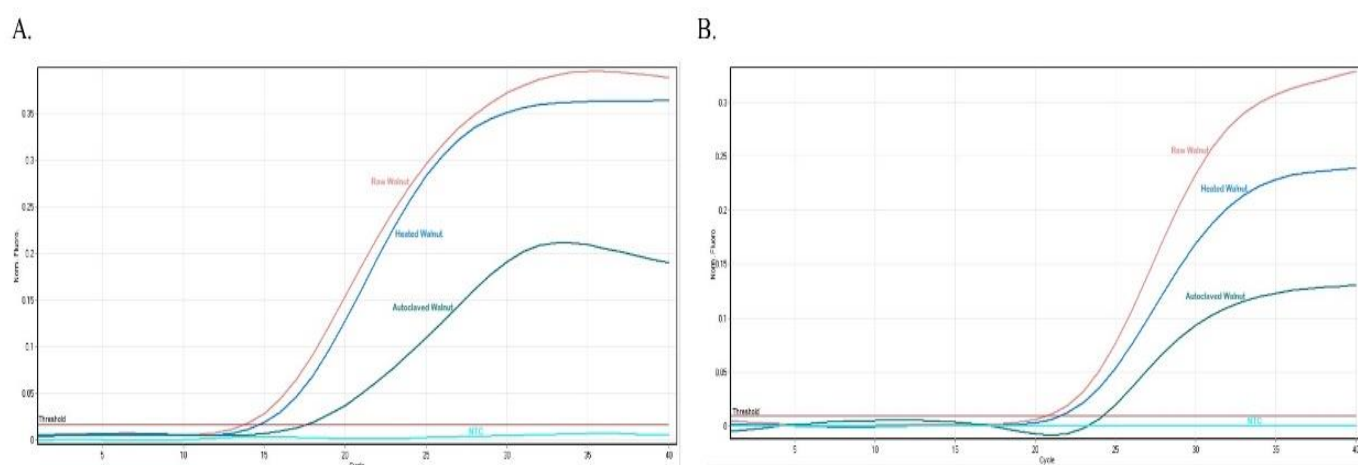
Figure 3. Effects of thermal processing on the detectability of pure walnut DNA. (A) Representative amplification curves of the IAC gene in untreated, dry heated and autoclaved walnut samples; and (B) corresponding amplification curves for the Jug r 2 gene. The increase in Ct values and decreased fluorescence plateau in autoclaved samples reflect partial DNA fragmentation induced by high-pressure steam sterilization. NTC: No-template control.
