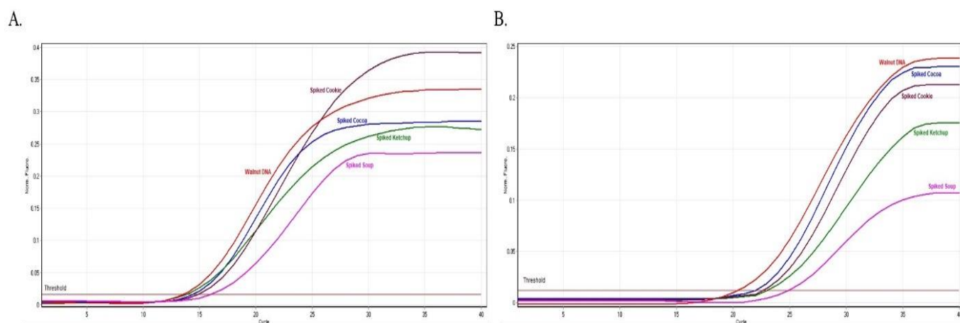
Figure 2. Effects of food matrix on the duplex qPCR assay performance. Representative amplification curves for (A) IAC and (B) Jug r 2 gene in walnut DNA (reference) and spiked complex food matrices (cookies, soup, ketchup and cocoa). The observed shifts in Ct and variations in the fluorescence intensity reflect the presence of matrix-derived inhibitors.
