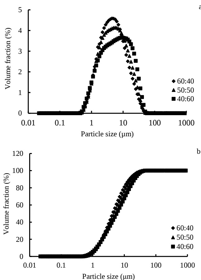
Figure 2. Pattern of particle size distributions of W_1/O/W_2 emulsions prepared at three ratios of W_1/O:W_2 and used for Lactobacillus casei encapsulation (a) and S-shaped curves for cumulative particle size distribution of the W_1/O/W_2 emulsions (b)
