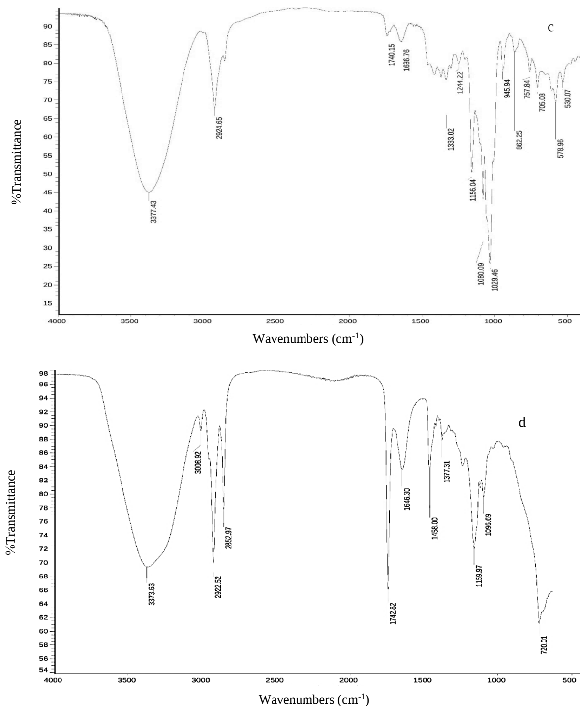
Figure 3. Fourier Transform Infrared spectroscopy spectra of Lactobacillus casei (a), pure form of the β-cyclodextrin powder (b), inclusion complex (IC) in the powder form (c), and W 1 /O/W 2 double emulsion at 60:40 ratio of W 1 /O: W 2 (d)
