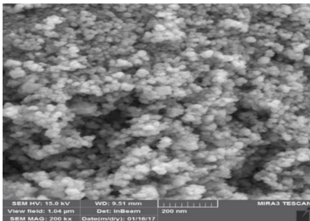
Figure 2. Scanning electron microscopy of the silver nanoparticle synthesis using \text{NaBH}_4
