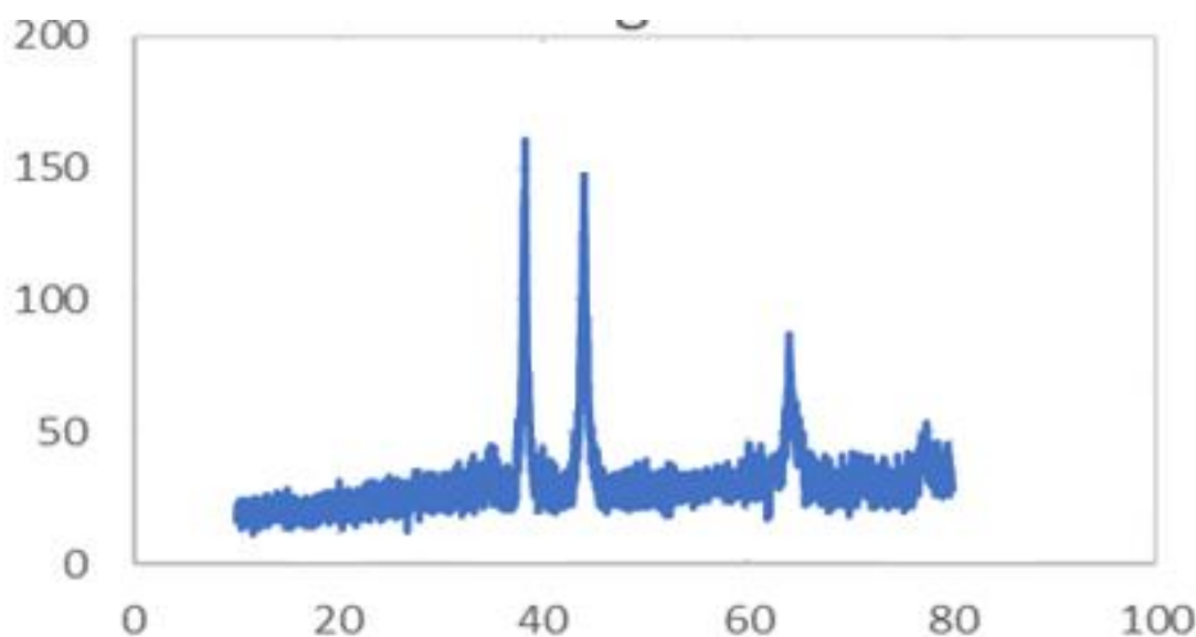
Figure 4. The X-ray diffraction diagram of the produced silver nanoparticles
